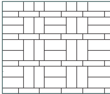
29. Basket Weave 8 x 16 in.
