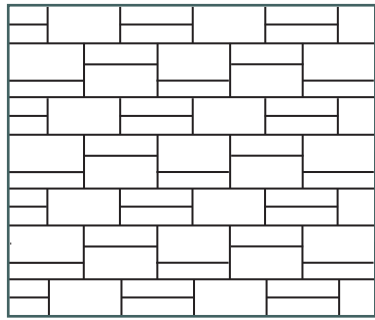
7. Coursed Ashlar 4 x 16, 8 x 16 in.
