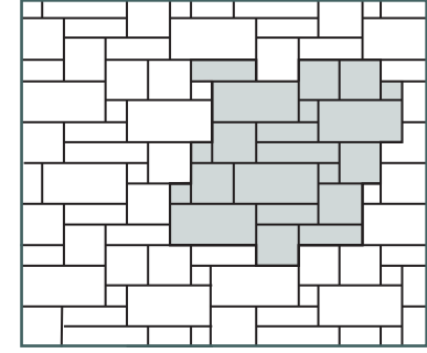
46. Patterned Ashlar 4 x 4, 4 x 12, 4 x 16, 8 x 8, 8 x 16 in.
