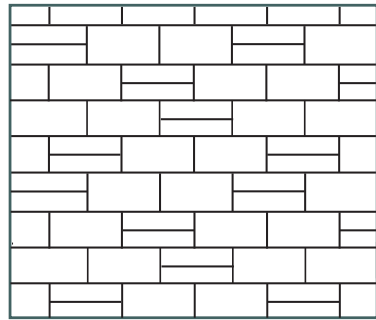
12. Coursed Ashlar 4 x 16, 8 x 16 in.
